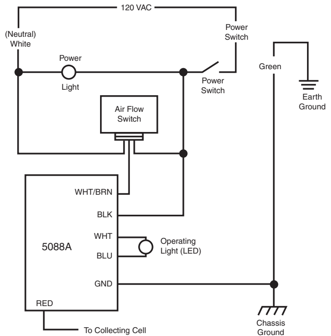
Figure 1. Typical System Wiring Diagram
