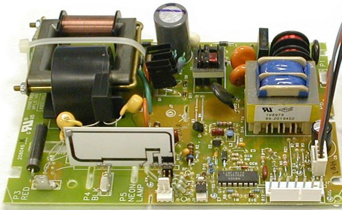
Series 2 Power Supply
