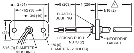
Fig. 1. C7046A,B,C,D Air Temperature Sensor dimensions in in. (mm).
