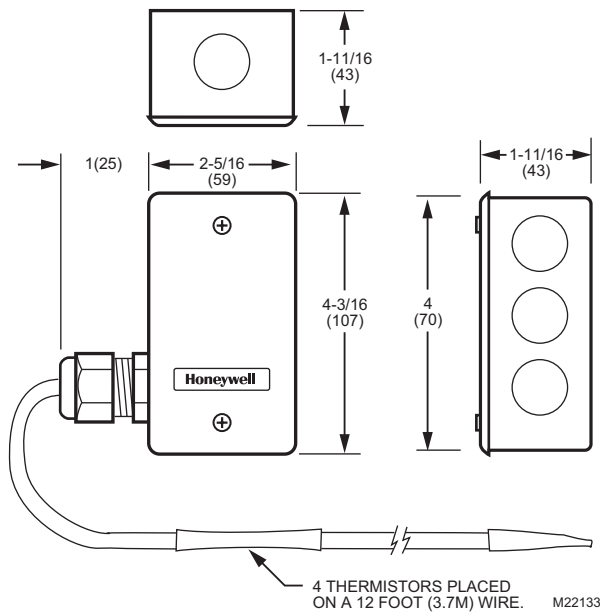
Fig. 9. C7031J, C7041J dimensions in in. (mm).
