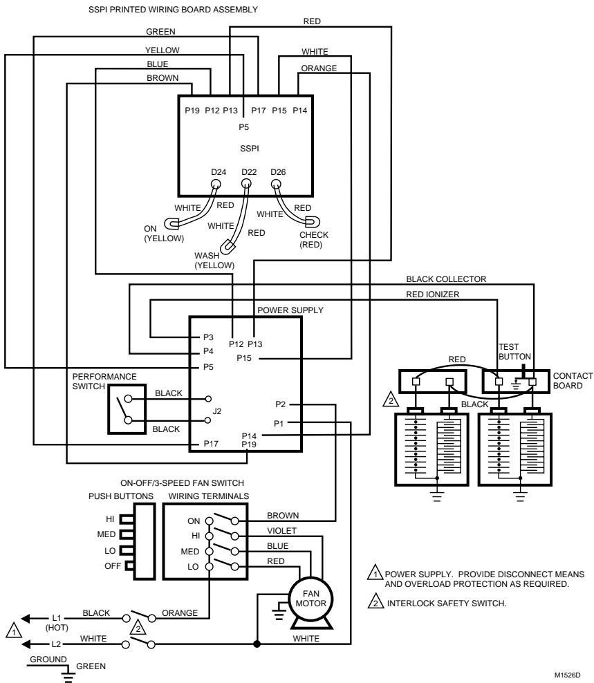
Fig. 11A. Past F90 schematic diagram.
