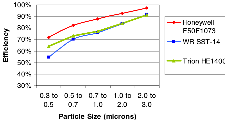
Fractional Efficiency 16" x 25 (1400 cfm)
