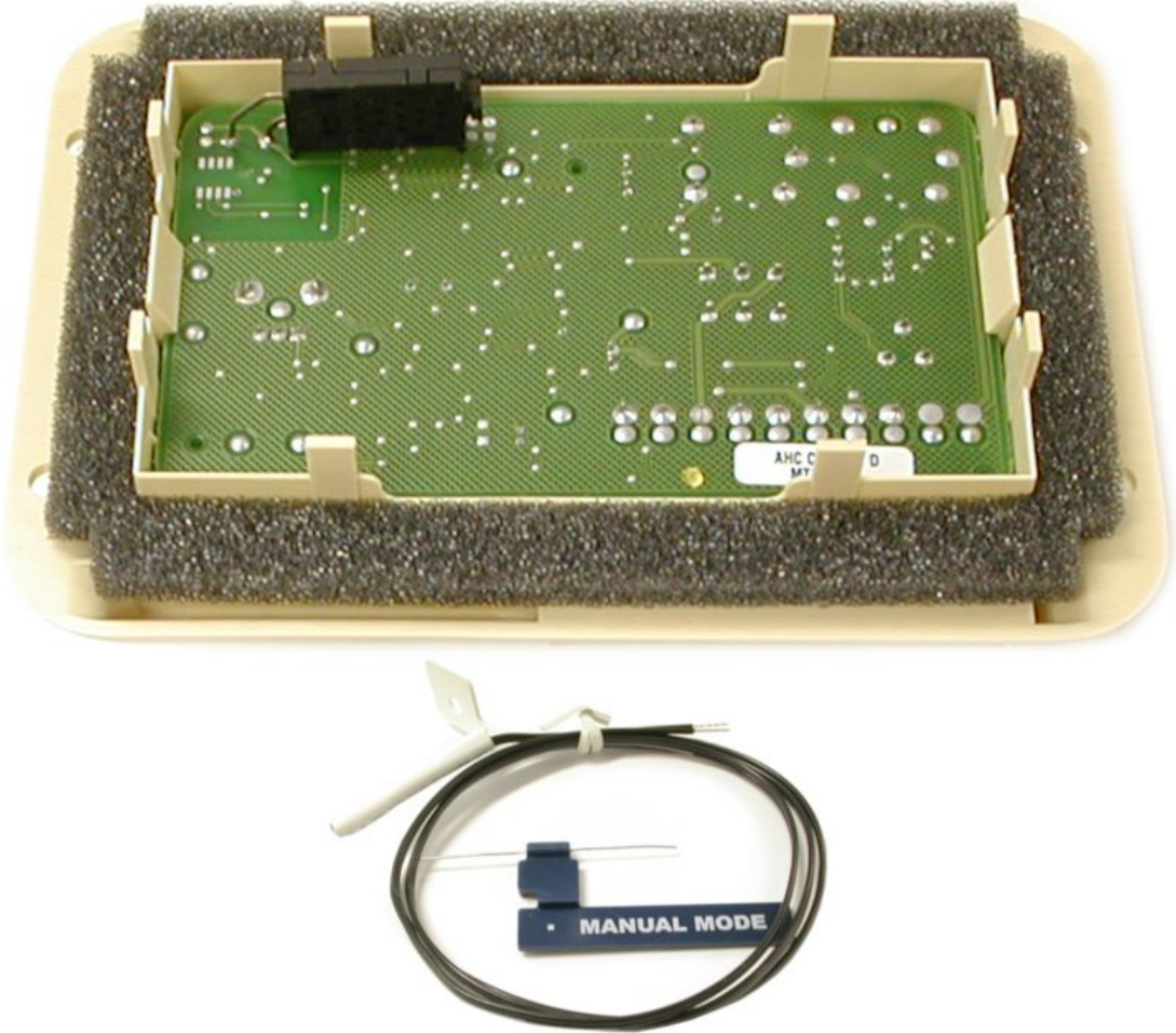
Backside View with Outdoor Temperature Sensor and Manual Mode Resistor
